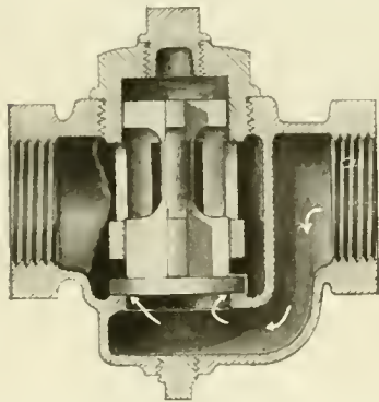
GREENWOOD BOILER CHECK VALVE.
